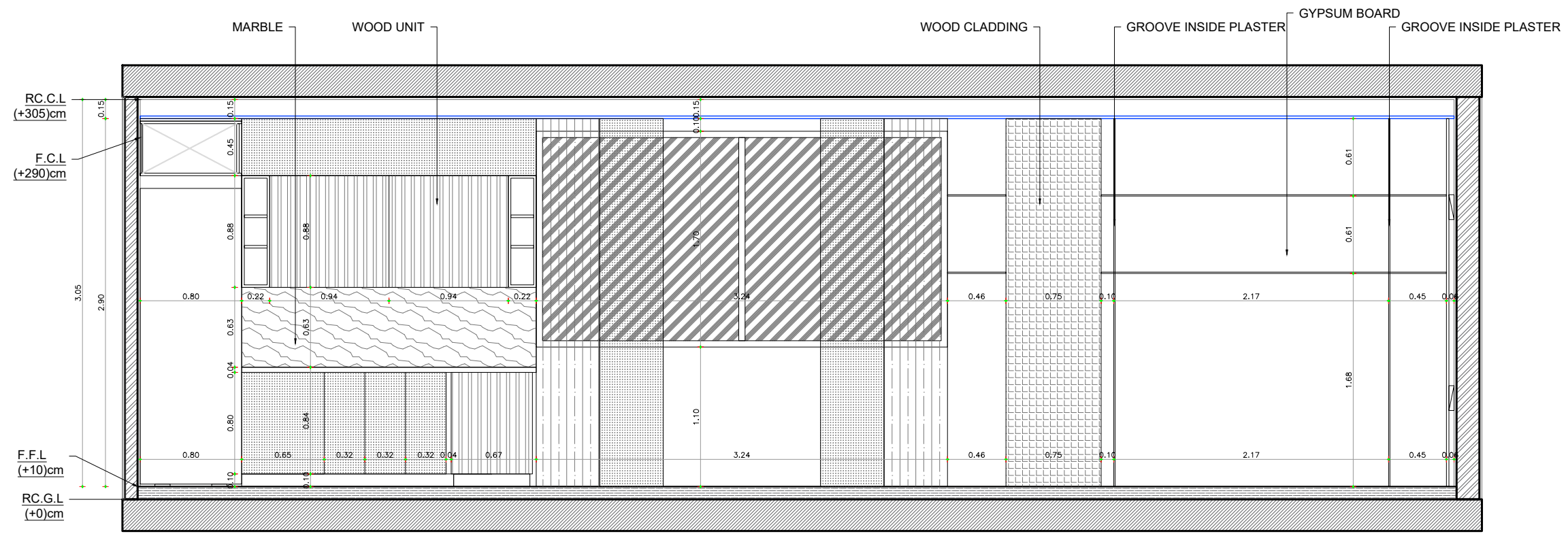
LIVING ROOM&KITCHEN SECTION (4)
